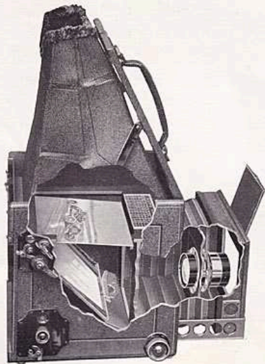
Sectional Illustration showing Graflex Principle
