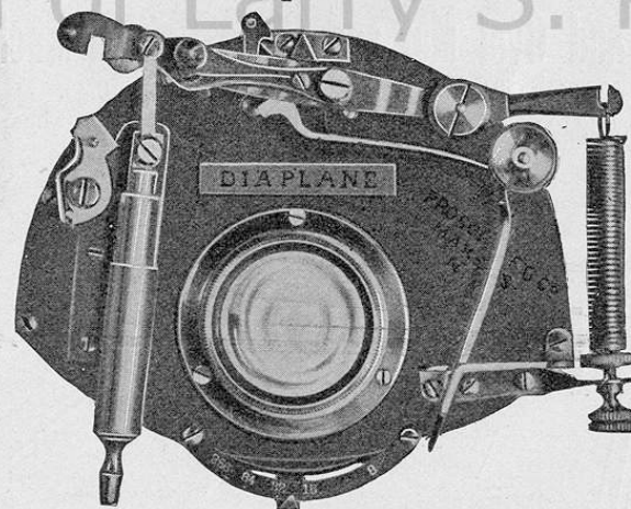
DIAPLANE II SHUTTER.
