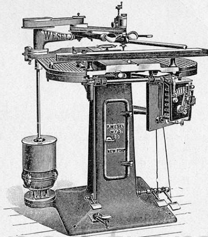
Wesel Radial Arm Routing Machine, with Direct Connected Motor.
