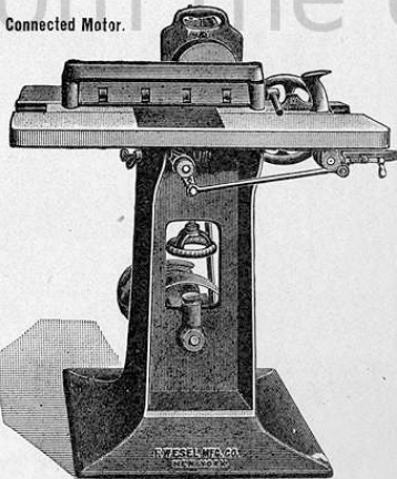
Photo-Engravers' Beveling Machine.
