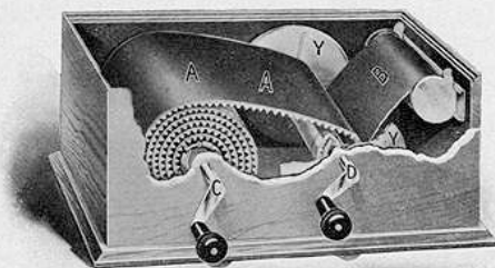
BOX FOR WINDING PROTECTING APRON AND FILM TOGETHER
